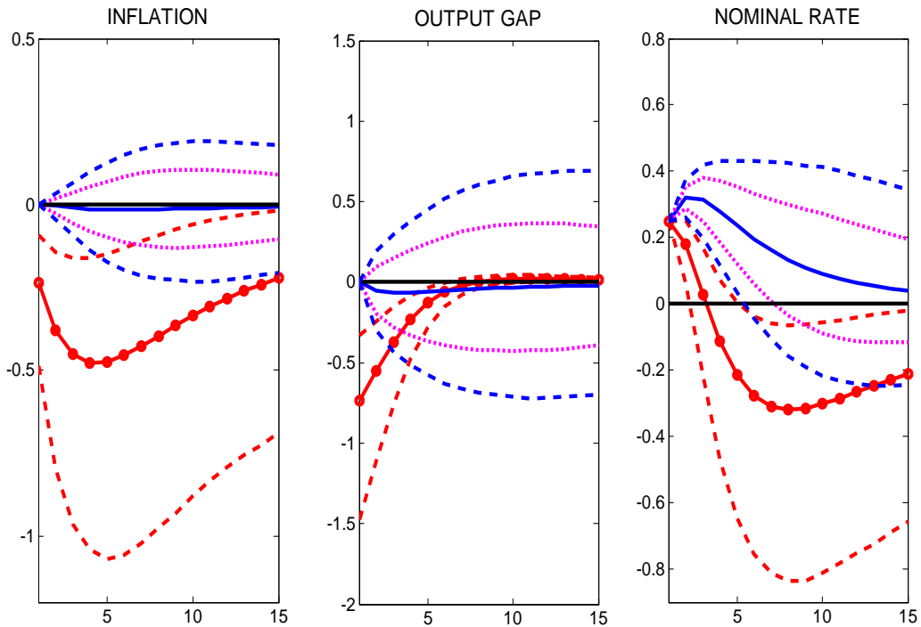
Figure 11: Measurement errors in the estimation of the DNK framework. Circled red lines: DNK Bayesian mean impulse responses; Dashed red lines: 90% credible sets. Solid blue line: VAR mean impulse responses; Dashed blue lines: 90% confidence bands; Magenta dotted lines: 68% confidence bands. Moments computed the impulse response function distributions simulated by drawing 10,000 realizations of the vector of parameters of the DNK model, which is also used to generate the pseudo-data to feed the SVARs. Identification of the monetary policy shock via Cholesky decomposition (lower triangular matrix, ordering: inflation, output gap, nominal rate). VARs estimated with two lags. Serially and mutually uncorrelated a-priori Inverse Gamma(0.35,0.2) distributed measurement errors modeled in the estimation.
